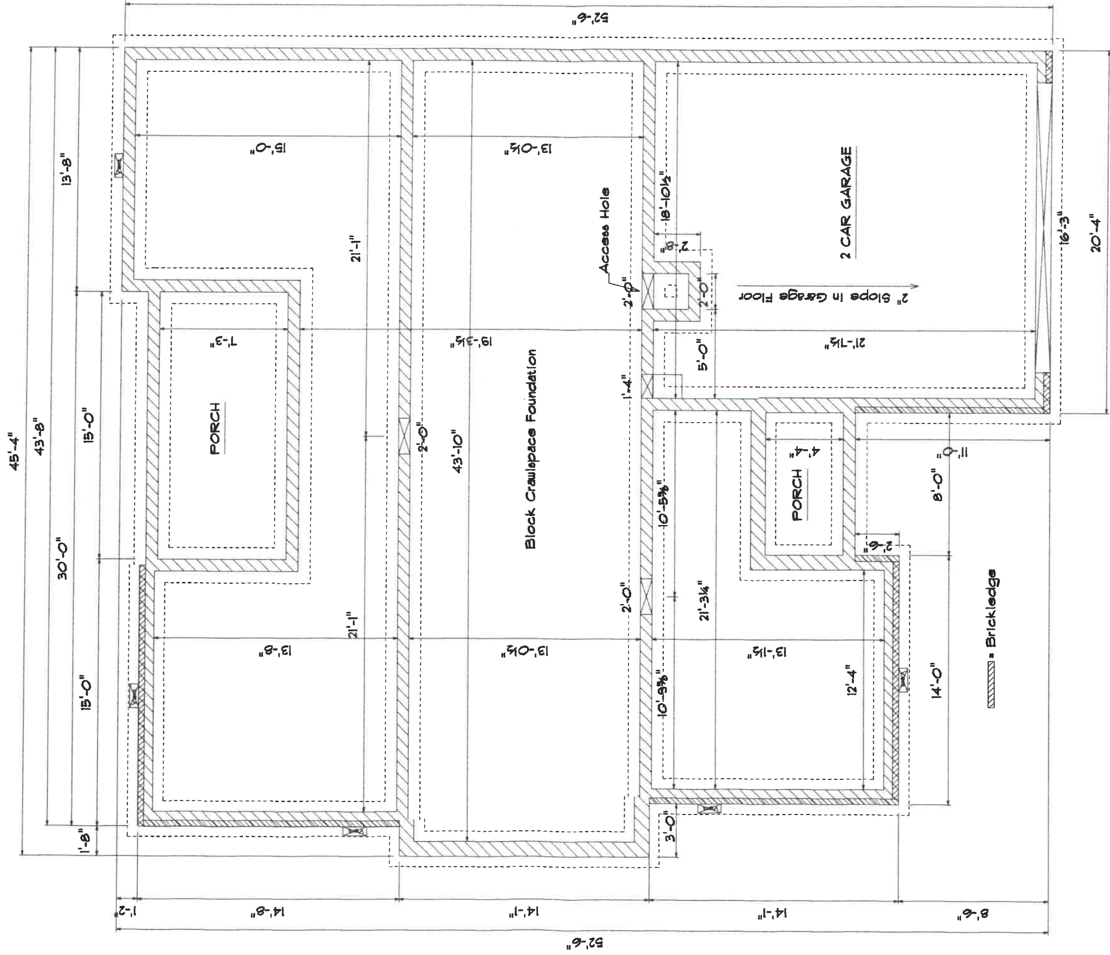
FOUNDATION PLAN
